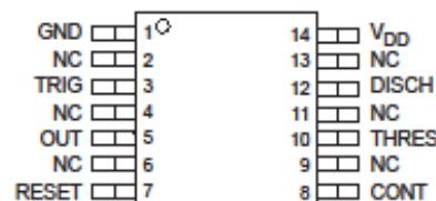
PW PACKAGE (TOP VIEW)
