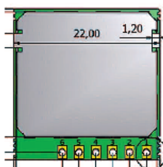
Figure 1. Pin numbering in the Fastrax UP501 module.
